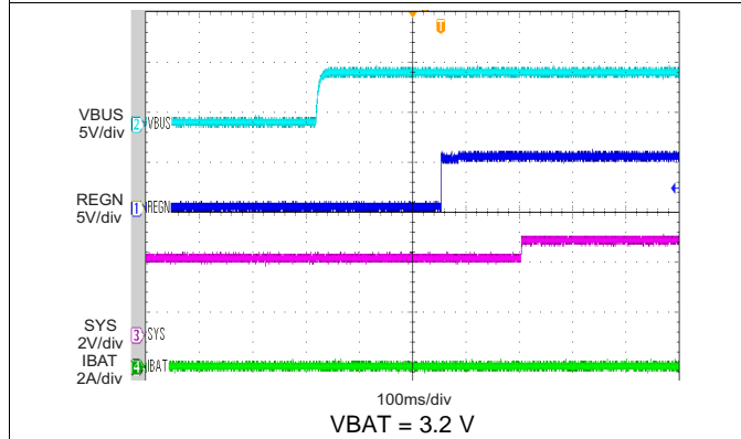
Figure 42. bq24296 Power Up with Charge Enabled
