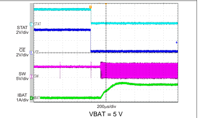
Figure 43. bq24297 Power Up with Charge Enabled
